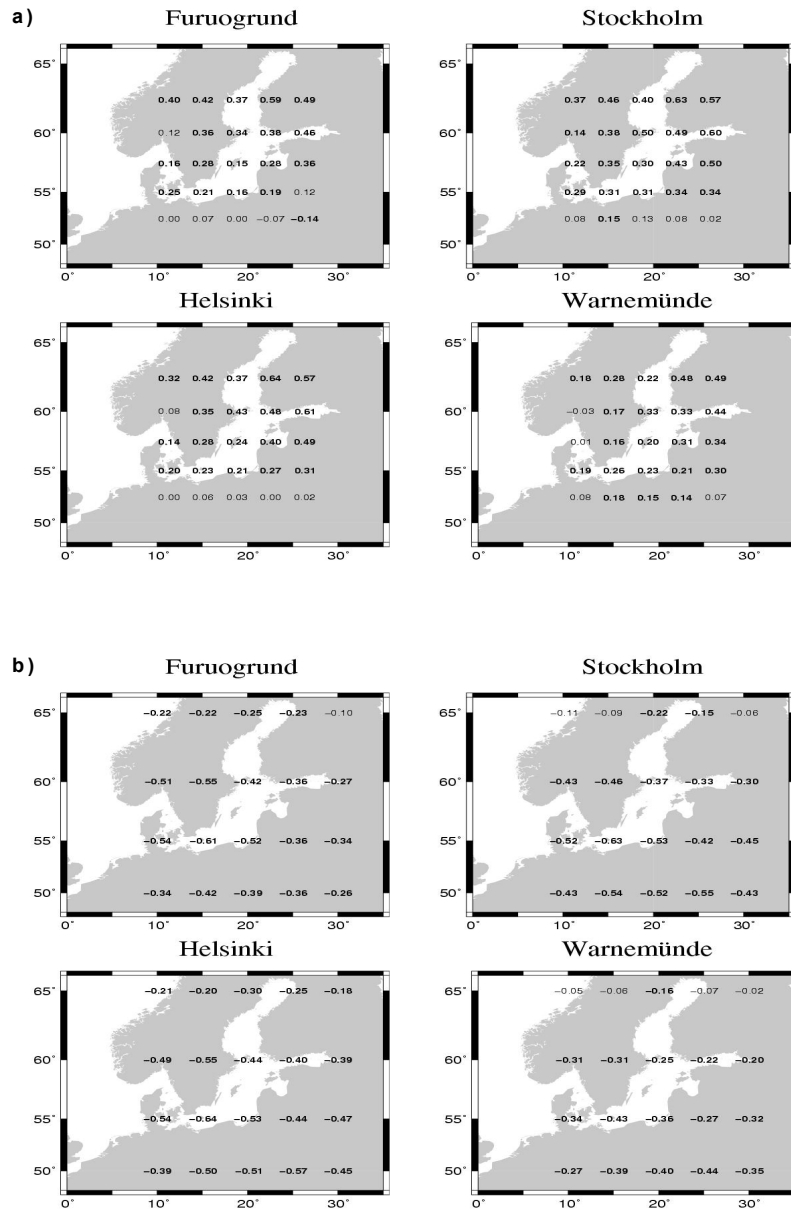
Fig. 2.11 Correlation patterns between (a) sea-level and precipitation and (b) sea-level and air-temperature in summer, 1900-1996. The 95% significance level is 0.14. Statistically significant correlations are bold-typed.
